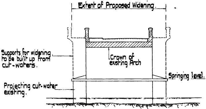
Fig. 207.—Method of Widening where existing Piers project.
